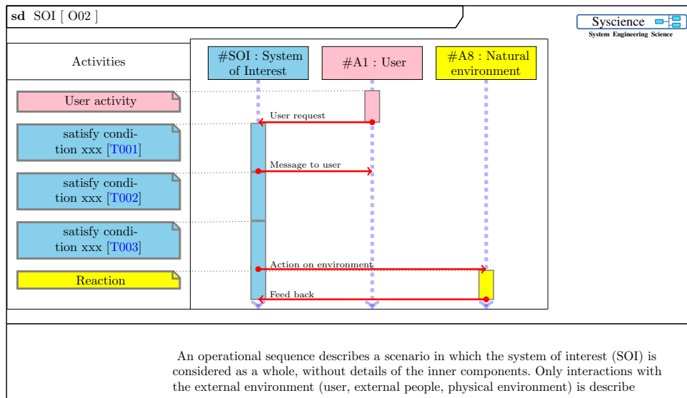
Figure 3: Sequence_O02
