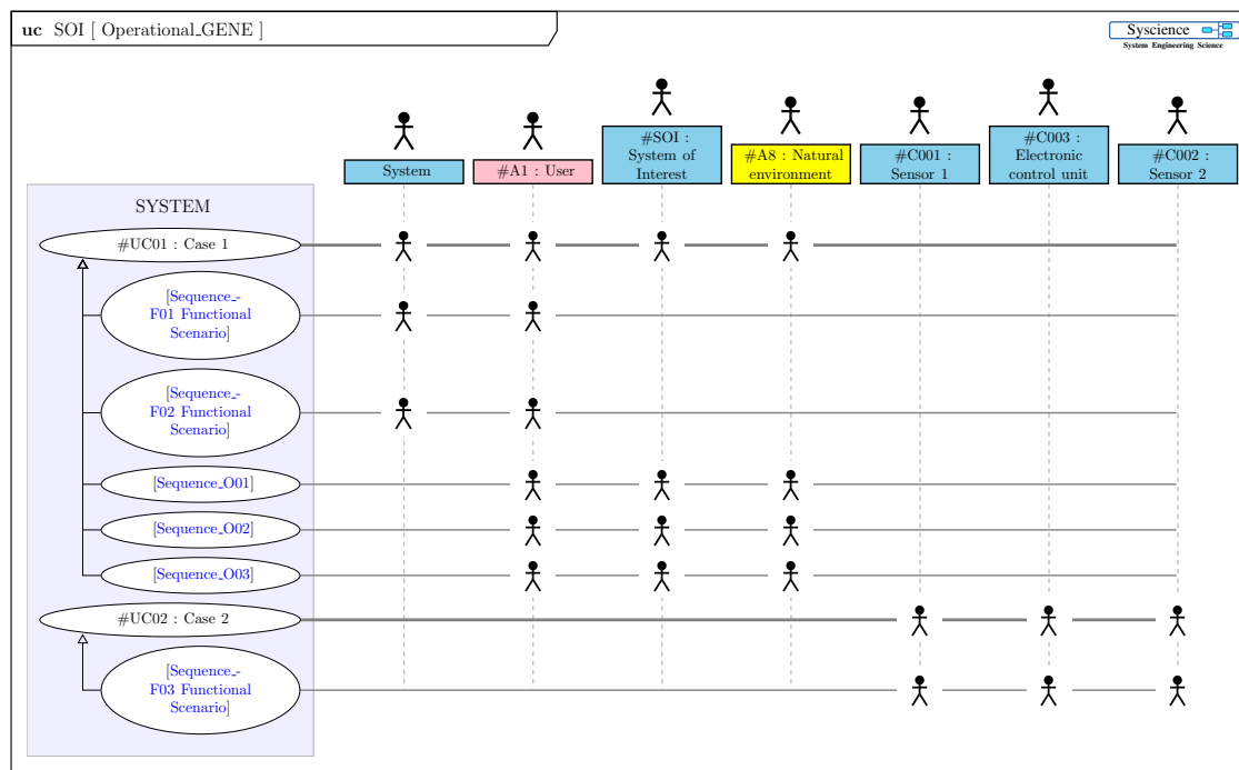
Figure 1: UseCase_Operational_GENE
