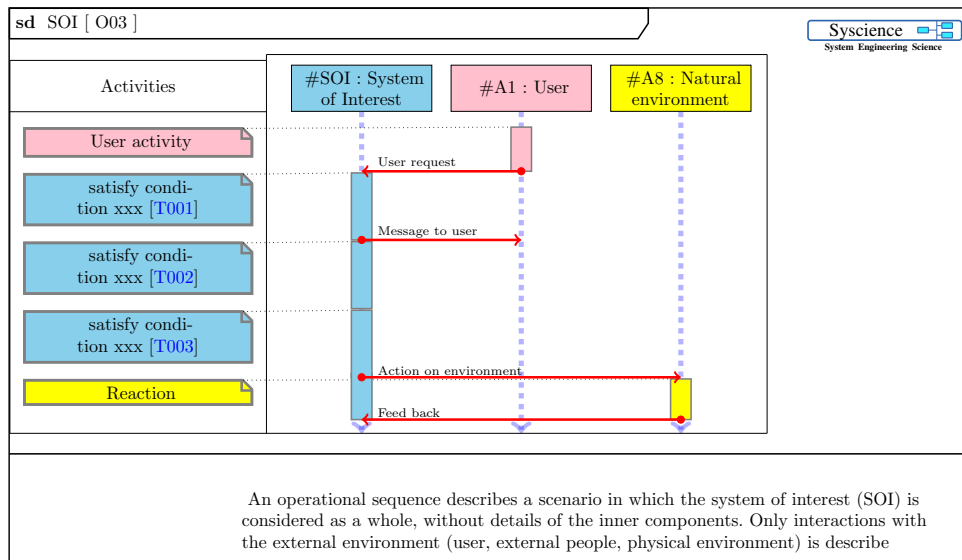
Figure 4: Sequence_O03
