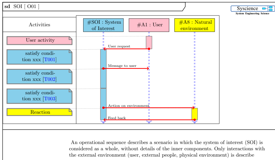
Figure 2: Sequence_O01
